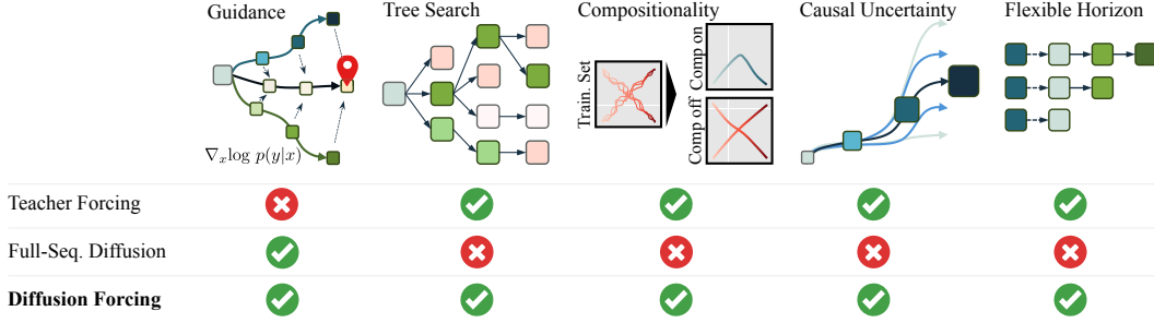
Figure 1: Diffusion Forcing capabilities. Today, different applications such as language modeling [6], planning [37], or video generation [32, 70] rely on either auto-regressive next-token prediction or full-sequence diffusion, according to their respective unique capabilities. The proposed Diffusion Forcing is a novel sequence generative model that enjoys key strengths of both model types.
